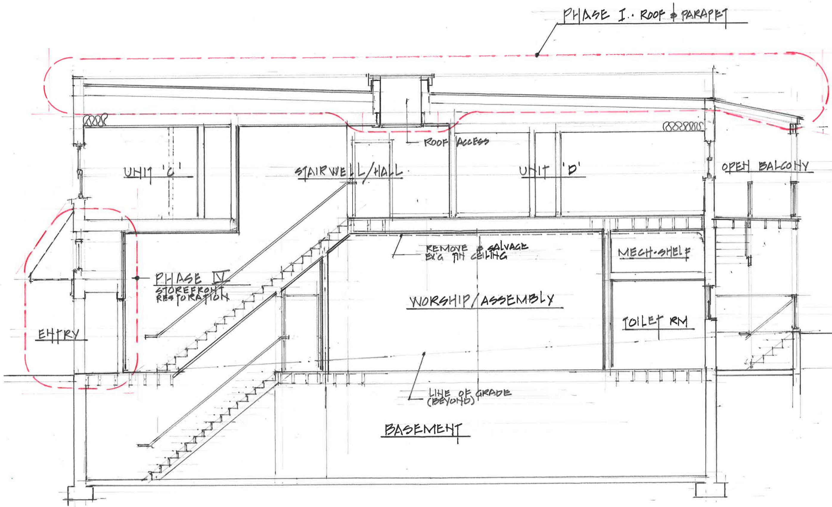
BUILDING SECTION A-A SCALE 3/16" = 1'-0"
